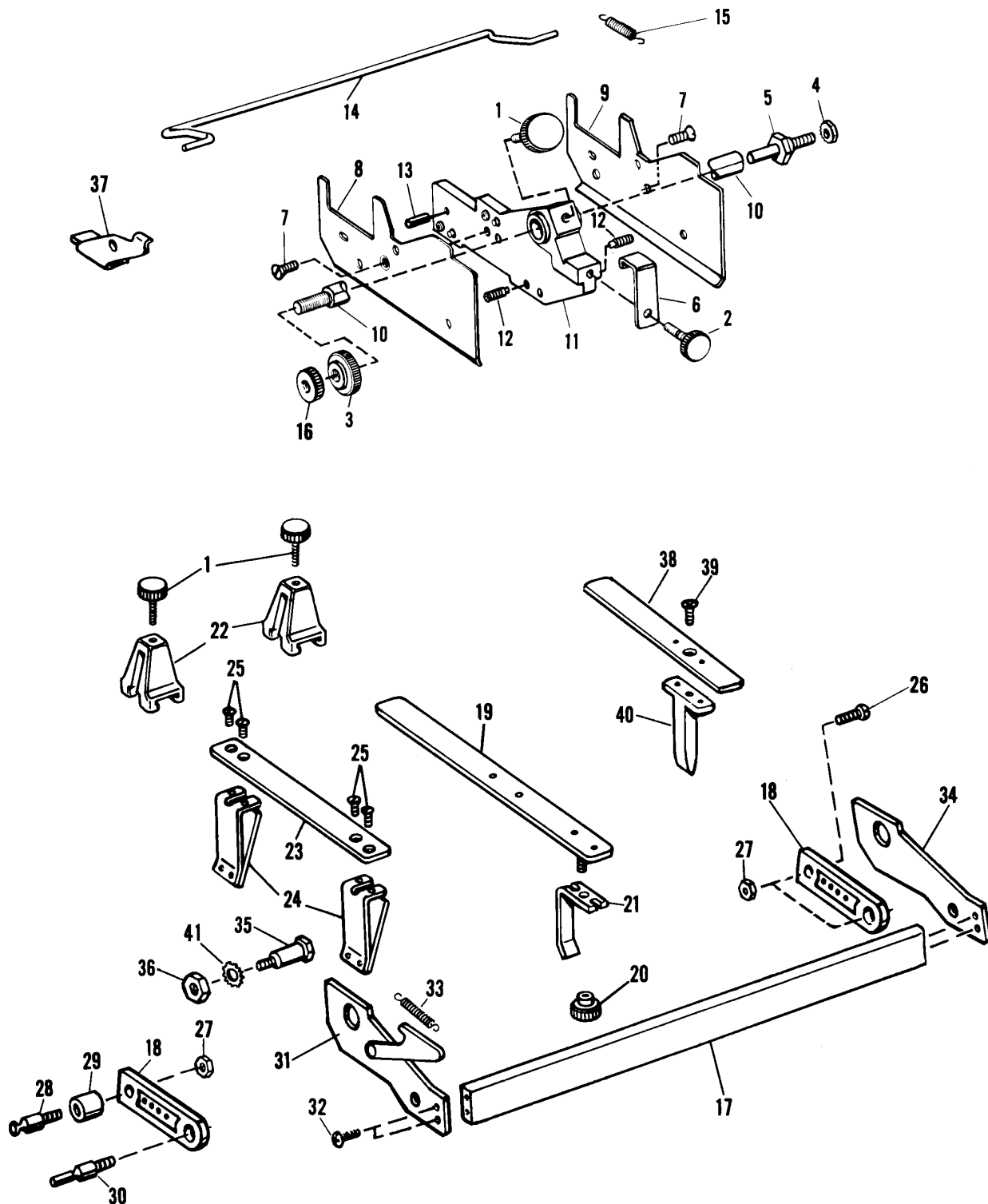
FIGURE 1 Paper Guides and Mounting Bar
