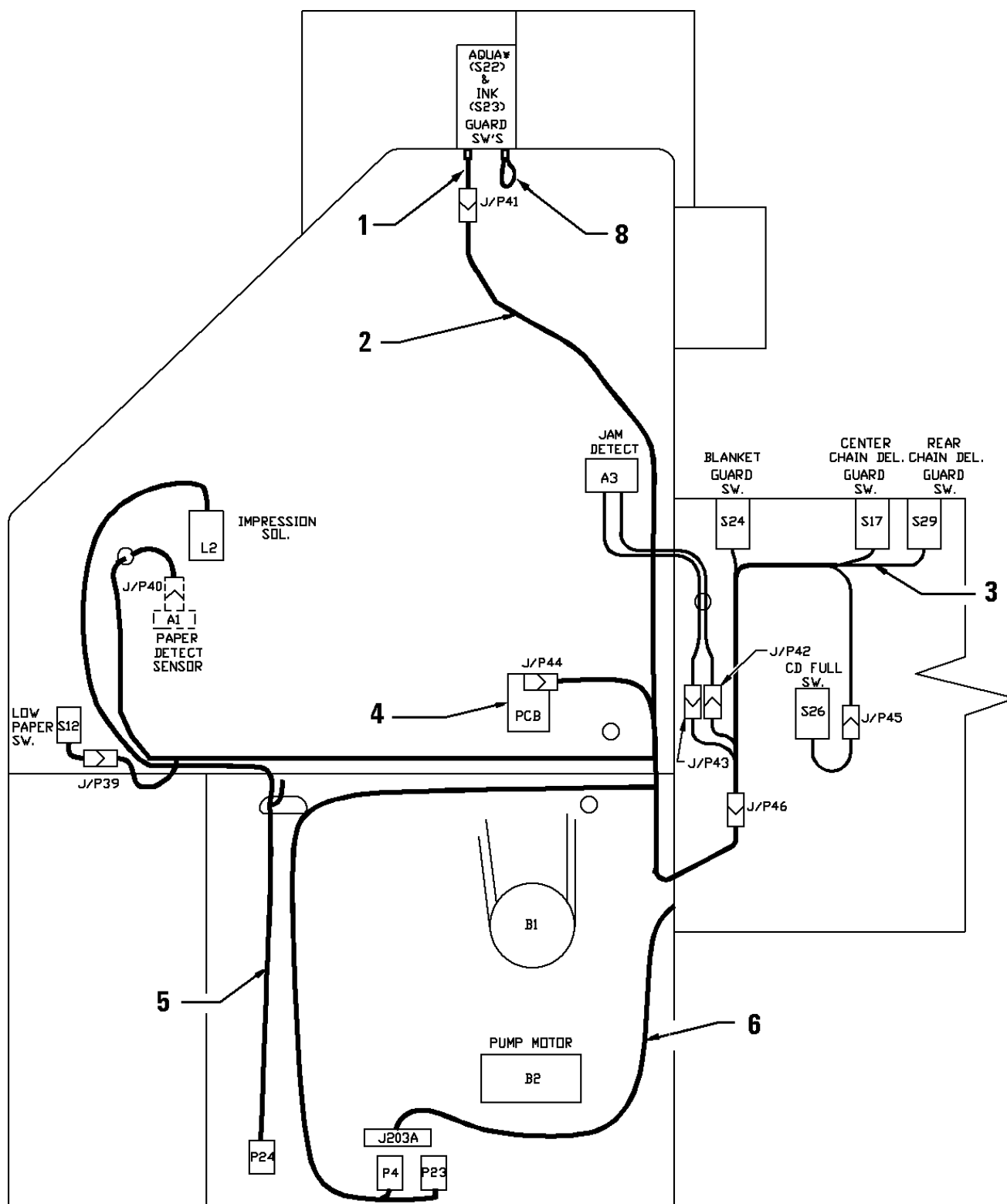
FIGURE 55 Wire Harness - N.O.S.
