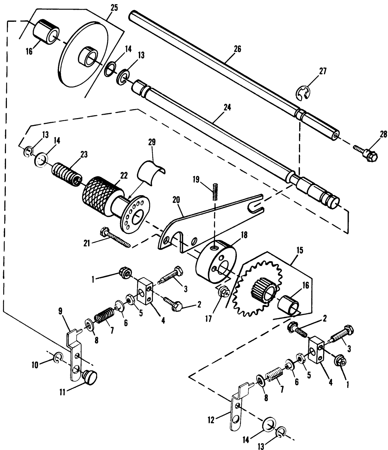
FIGURE 64 Idler Shaft Assembly
