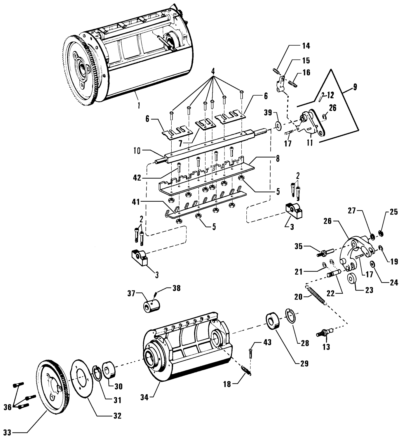
FIGURE 33 Impression Cylinder Assembly
