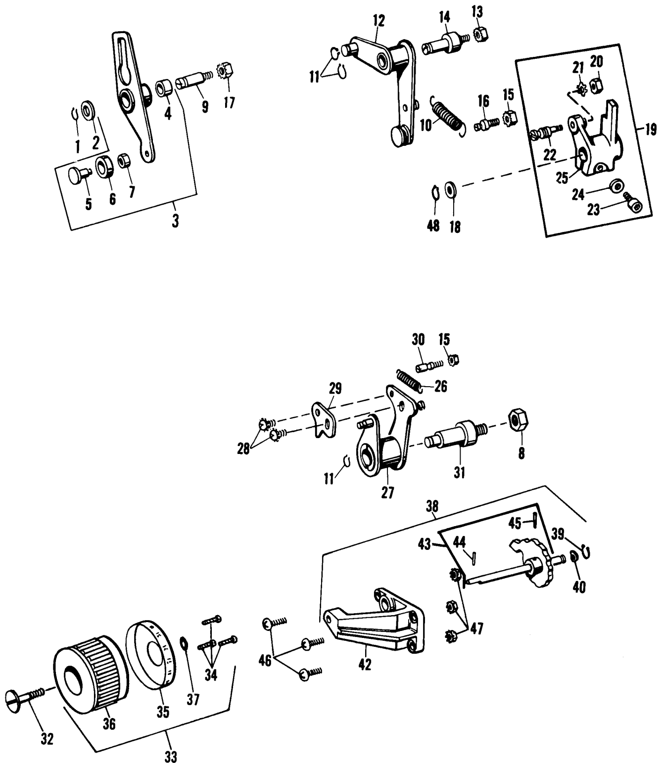
FIGURE 40 Buckle Adjusting and Lever Assemblies
