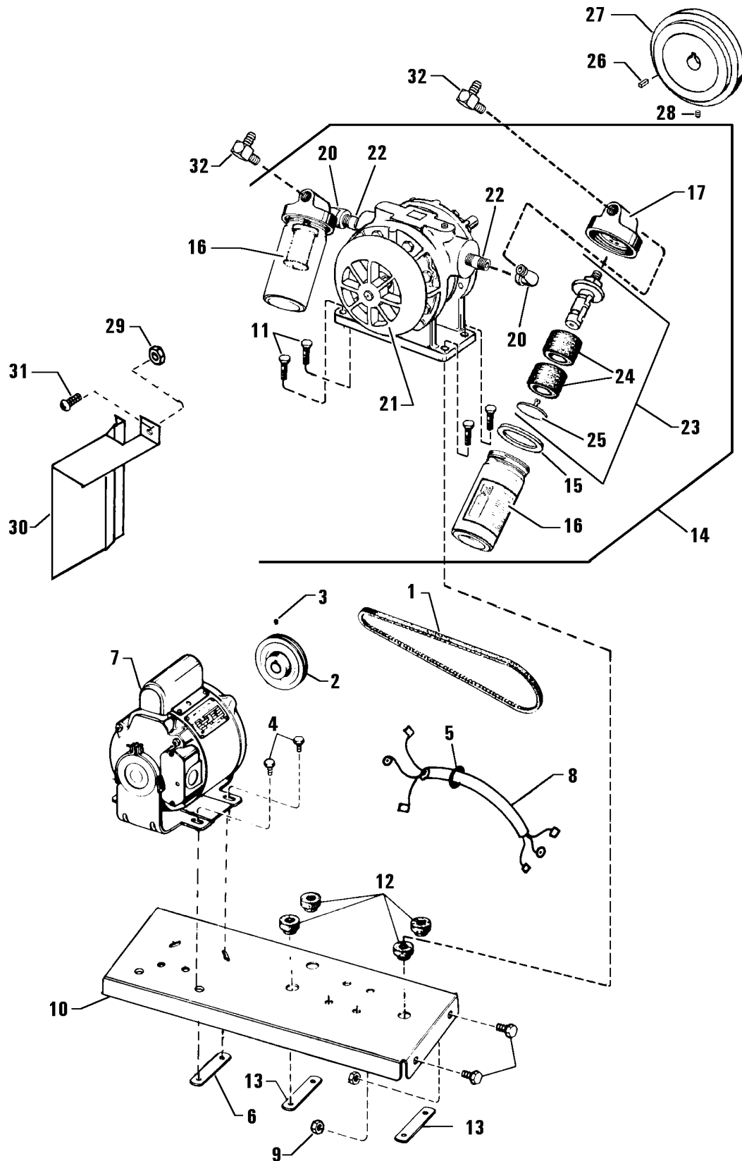
FIGURE 53 Compressor Assembly
