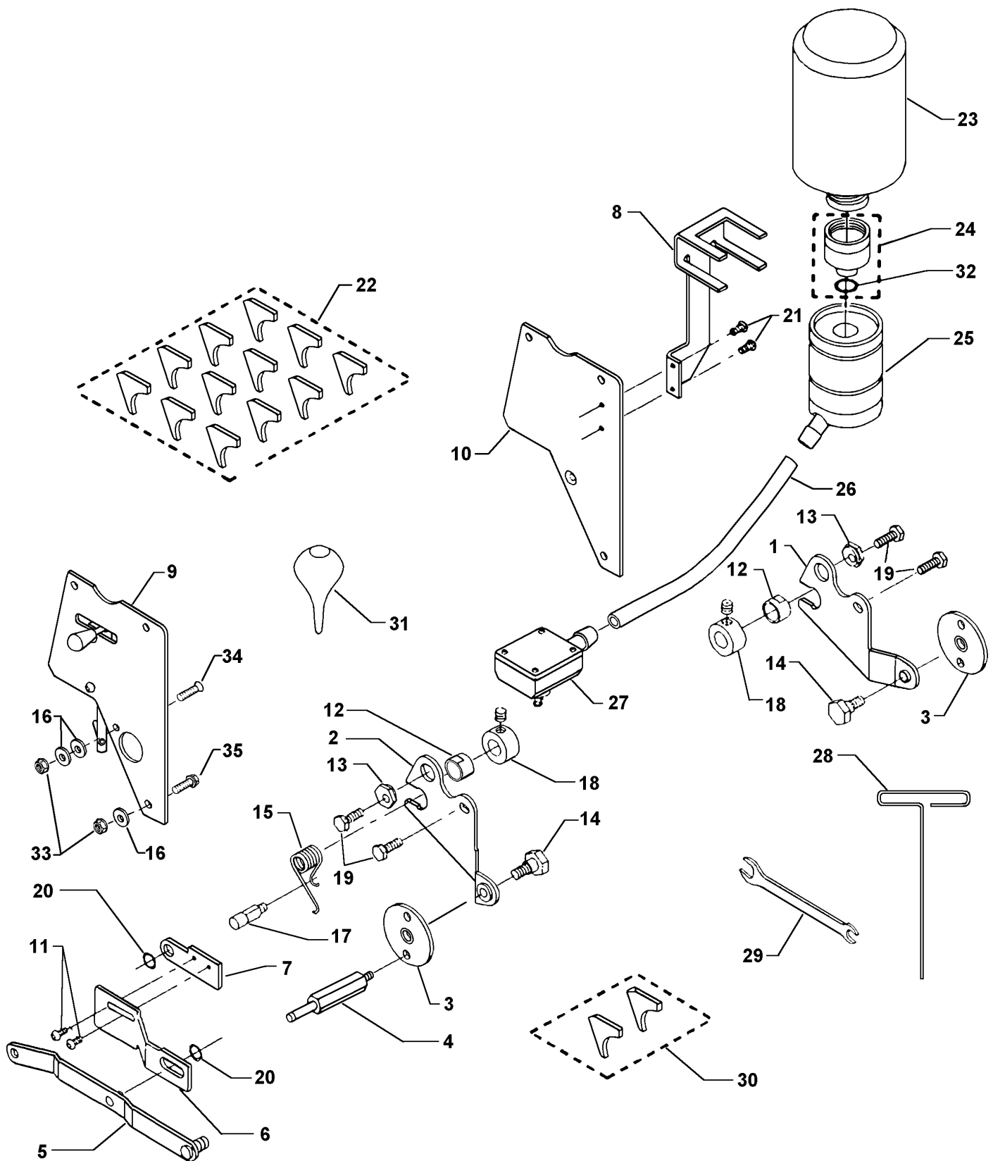
FIGURE 12B Non-Motorized Dampener Part II
