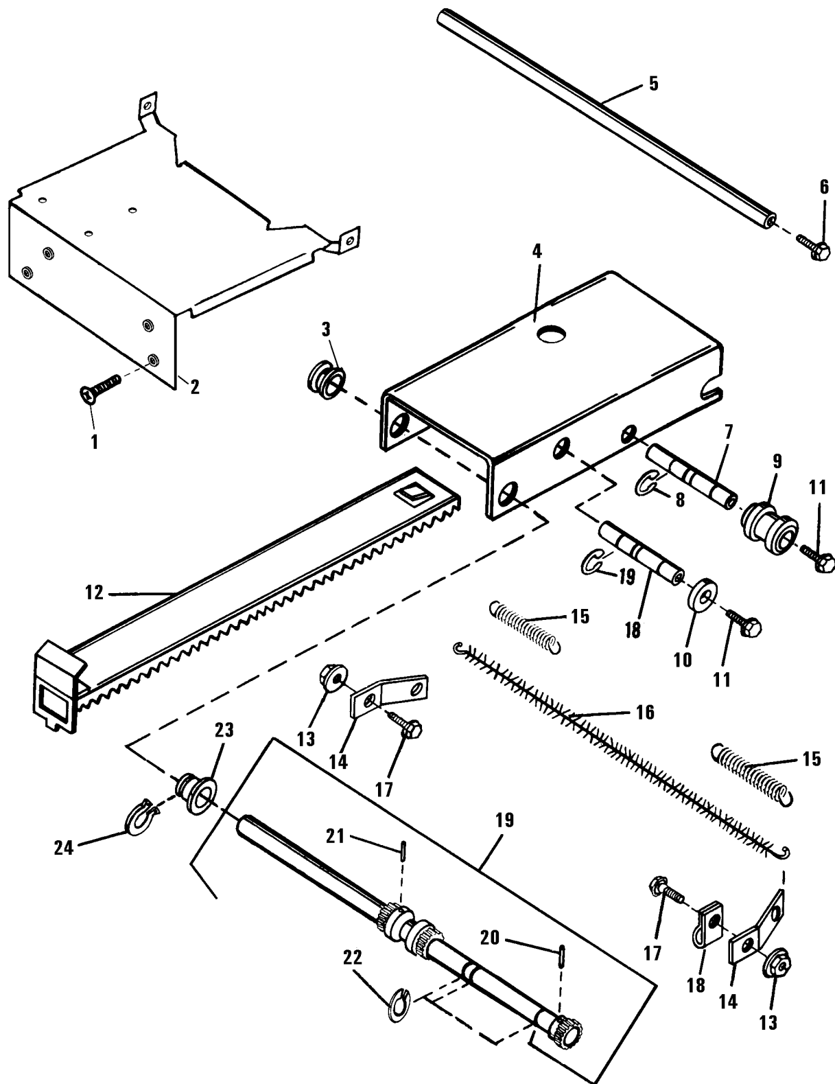
FIGURE 65 Back Jogger Mechanism - Part I
