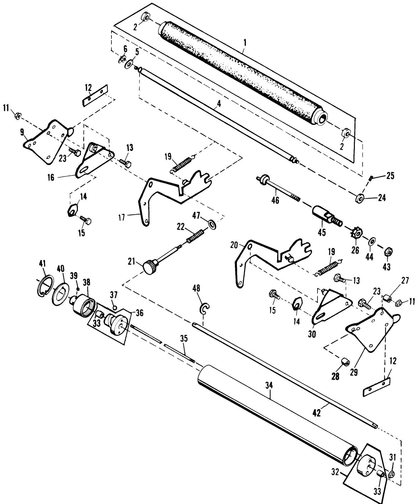
FIGURE 20 Form Roller - Third
