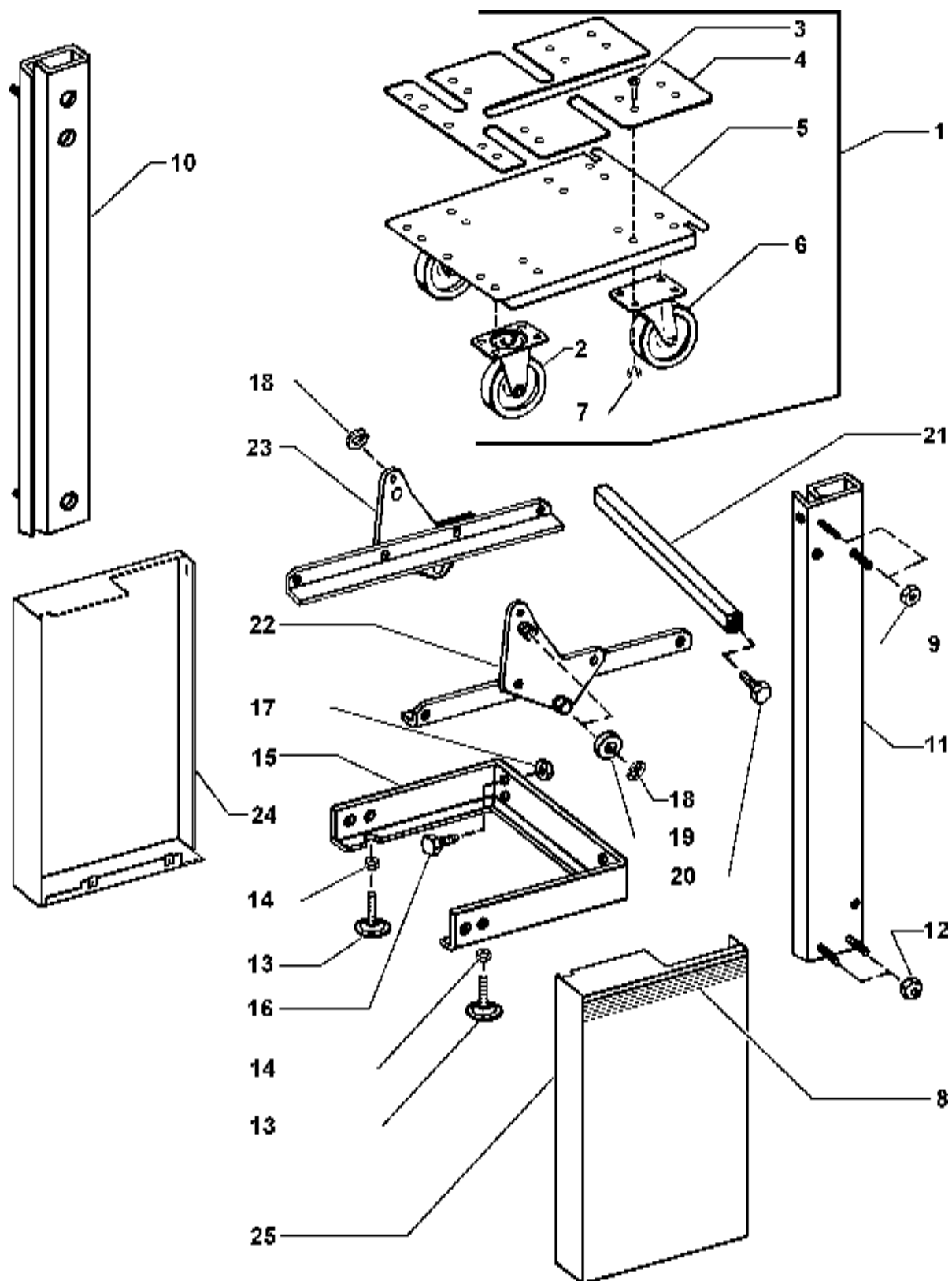
FIGURE 73 Dolly and Frame Assemblies
