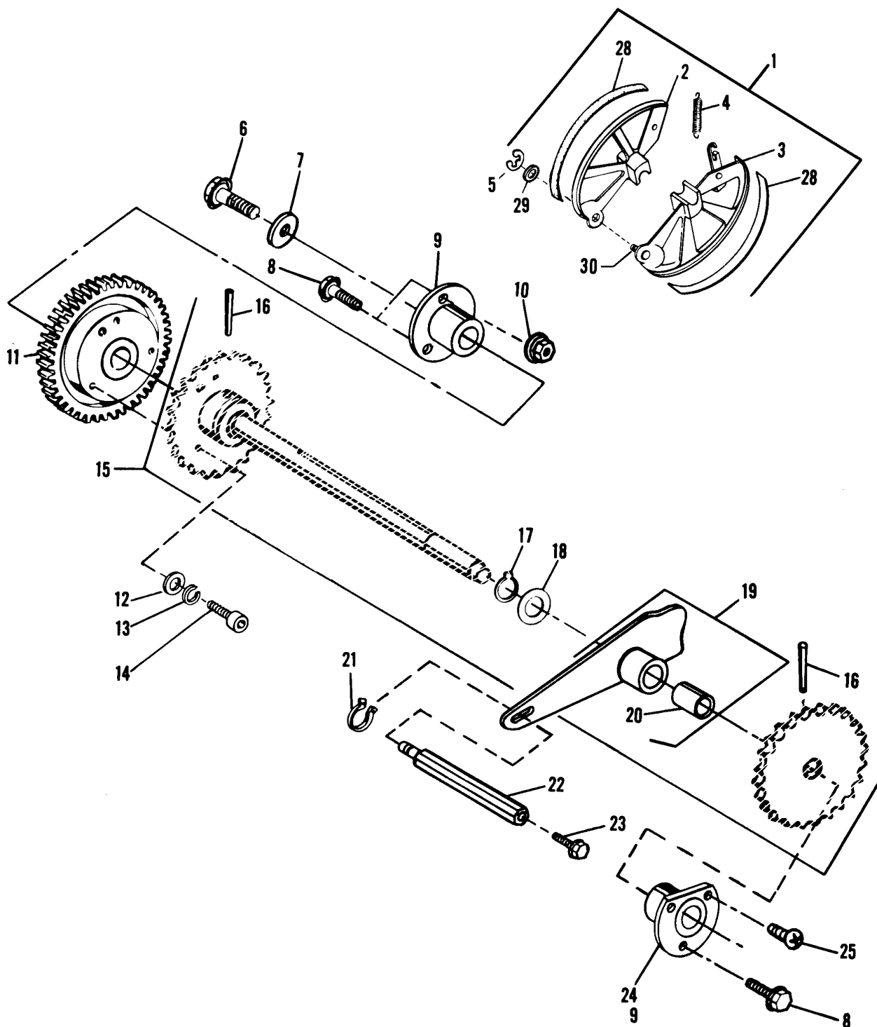
FIGURE 62 Sprocket Shaft and Paper Guides
